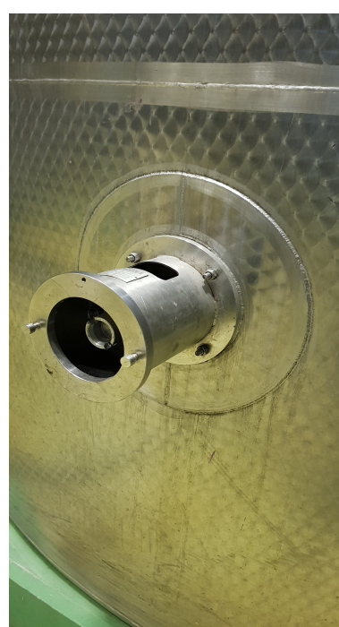
Above: Bayonet-type, portable drive mixer complete, tank bedestal assembly and bayonet coupler
