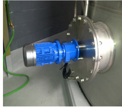
Chemical tank mixer with special hard faced mechanical seal & water flush
